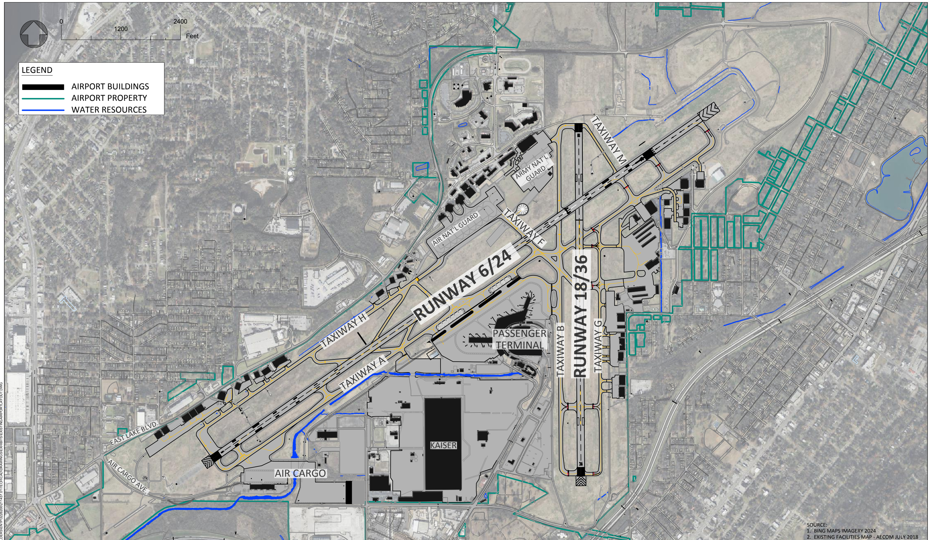
FIGURE A2 EXISTING AIRPORT LAYOUT
