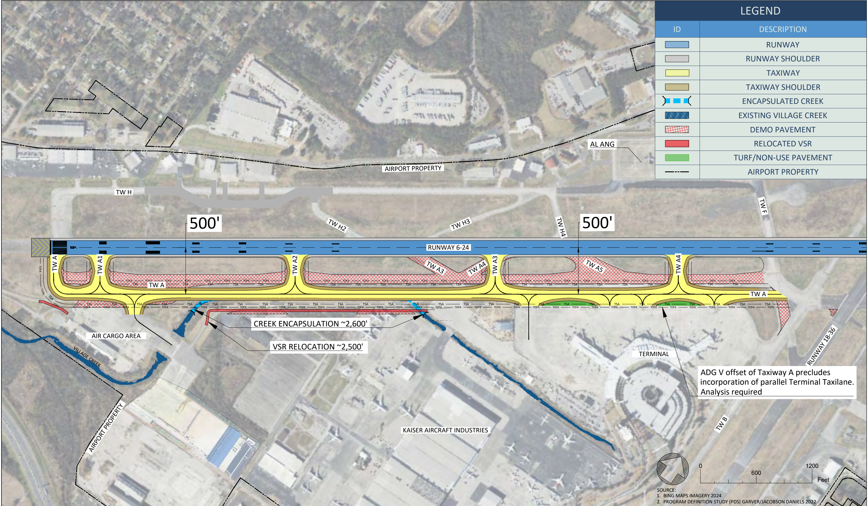
FIGURE B3 ALTERNATIVE 3a: VILLAGE CREEK ENCAPSULATION IN PLACE AND TAXIWAY A RELOCATION TO 500 FEET
