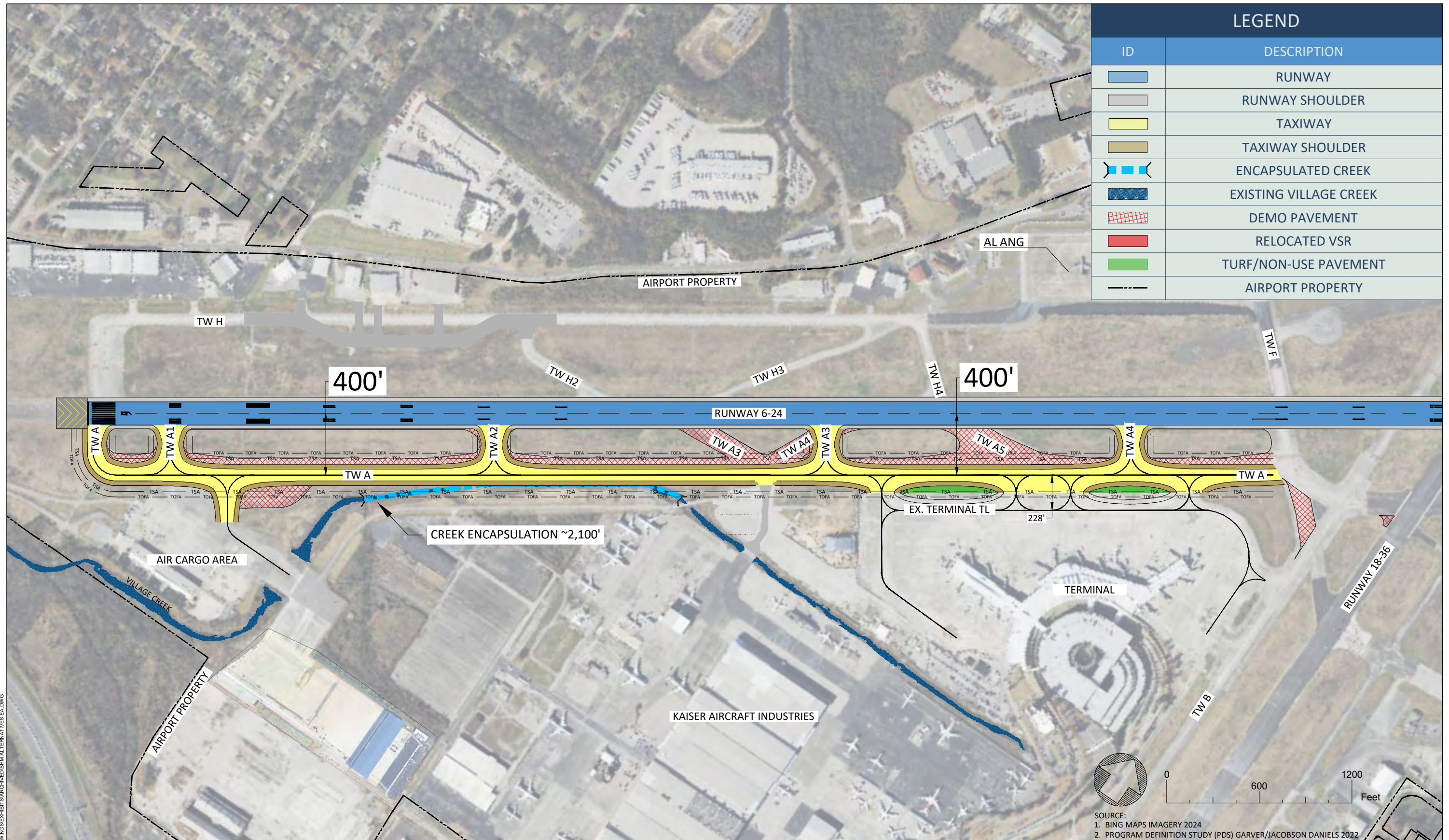
FIGURE B1 ALTERNATIVE 1: VILLAGE CREEK ENCAPSULATION IN PLACE AND TAXIWAY A RELOCATION TO 400 FEET
